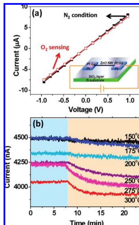
Figure 1. (a) I-V curves measured for the Ohmic contact device (OCD) in N 2 and O 2 atmospheres at 275 °C. Inset shows the schematic of the OCD. (b) The response curves of the oxygen detection recorded at different temperatures, ranging from 150 to 300 °C, for the OCD. The blue background denotes that the OCD was in the N 2 atmosphere and the pink background in the O 2 atmosphere.
