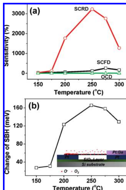
Figure 4. (a) Sensitivity versus system temperature for O_2 sensing at a response time of 500 s. Results collected from the OCD, SCD at forward bias (SCFD), and SCD at reverse bias (SCRD) were compared. (b) Derived SBH rise of the SCD at the reverse bias mode after the O_2 adsorption versus system temperature. Inset shows the schematic of the SCD at O_2 adsorption.
