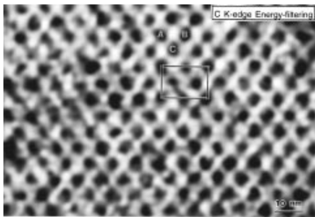
Figure 5. [110]_s energy-filtered TEM image of the carbon K ionization edge, showing the projected density of carbon along the [110]_s of the NCS.
