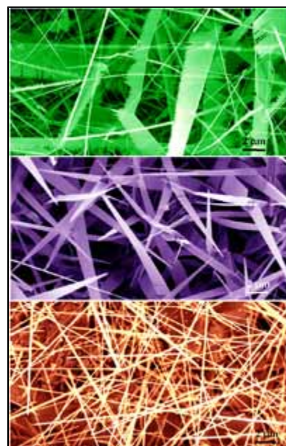
Scanning electron microscope images show nanosaws, nanobelts and nanowires of cadmium selenide grown using the vapor-liquid-solid process. 300 dpi JPG = 932.2 KB
